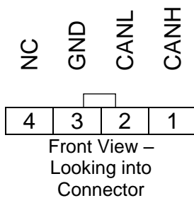
Figure 10: CAN_PORT
