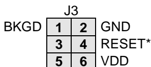
Figure 2: BDM_PORT Header
