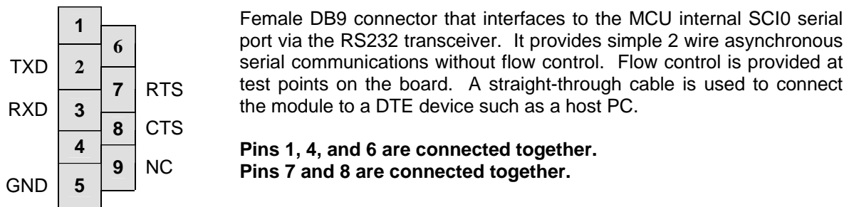
Figure 4: COM Connector
