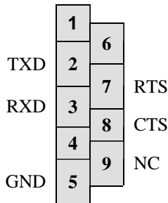
Figure 5: COM Connector
