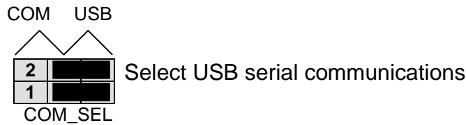
Figure 9: COM_SEL Option
