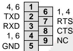
Figure 8: COM Connector
