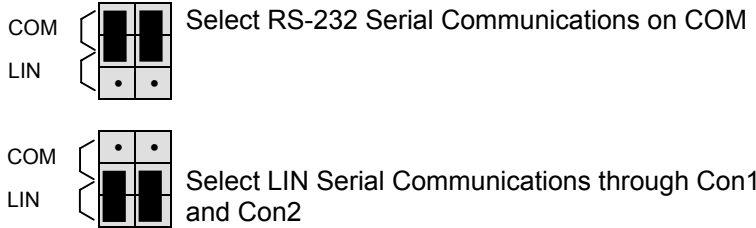
Figure 5: COM_SEL Jumper
