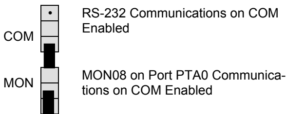
Figure 4: COM_MODE Jumper
