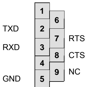
Figure 3: COM Connector
