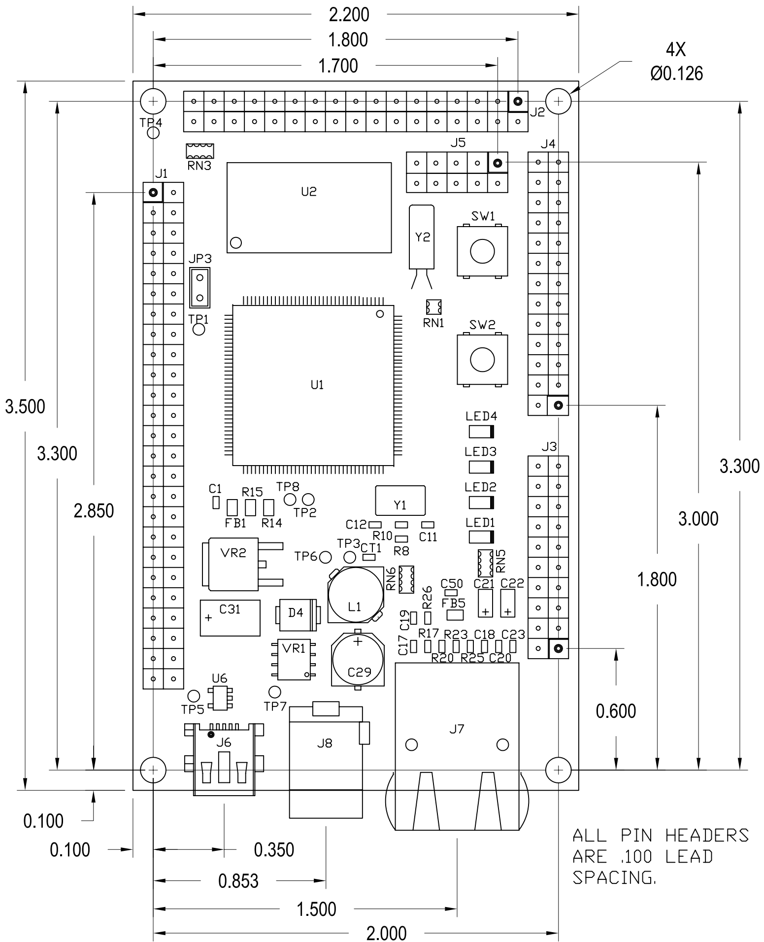
MECHANICAL DETAIL CMM-52259 AXM-0515 REV A AXIOM MANUFACTURING
